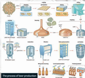
The process of beer production
